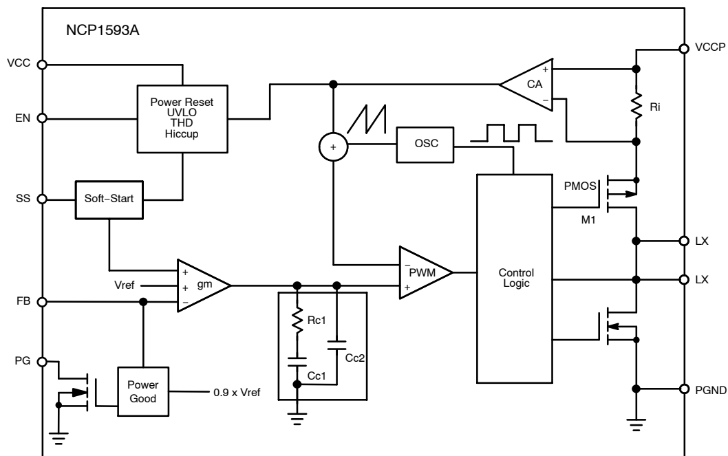
Figure 1. Block Diagram
