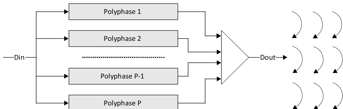
Figure 4.4. Polyphase Interpolator
