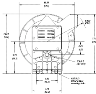
INDUSTRIAL DUTY CABLE REEL
