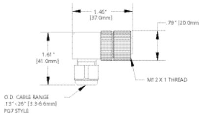
FEMALE 90°
