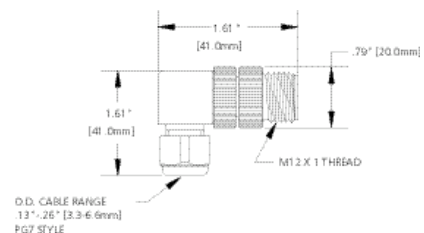
MALE 90°
