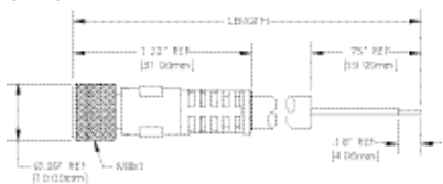
FEMALE STRAIGHT
