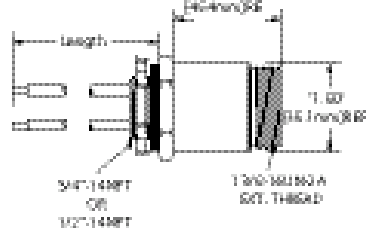
MALE RECEPTACLE
