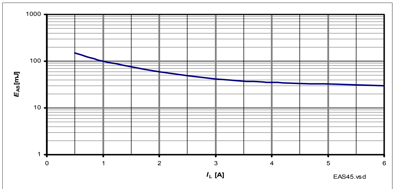
Figure 12 Maximum Energy Dissipation Single Pulse, T_{J(0)} = 150^\circ\text{C} ; V_S = 13.5\text{V}
