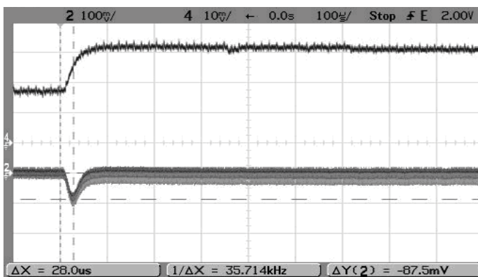
Step Load Transient Response (Vin=12V, Vout=2.5V, Clad=0, Iout=3A to 6A) Trace 2=Vout, 100 mV/div. Trace 4=Iout, 2A/div.
