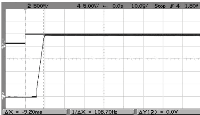
On/Off Enable Delay (Vin=13.8V, Vout=2.5V, Iout=6A, Clad=0) Trace 4=Enable, Trace 2=Vout
