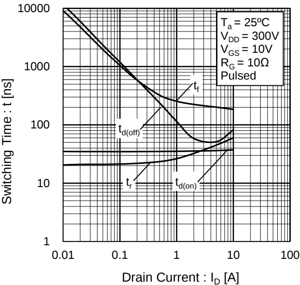
Fig.20 Switching Characteristics
