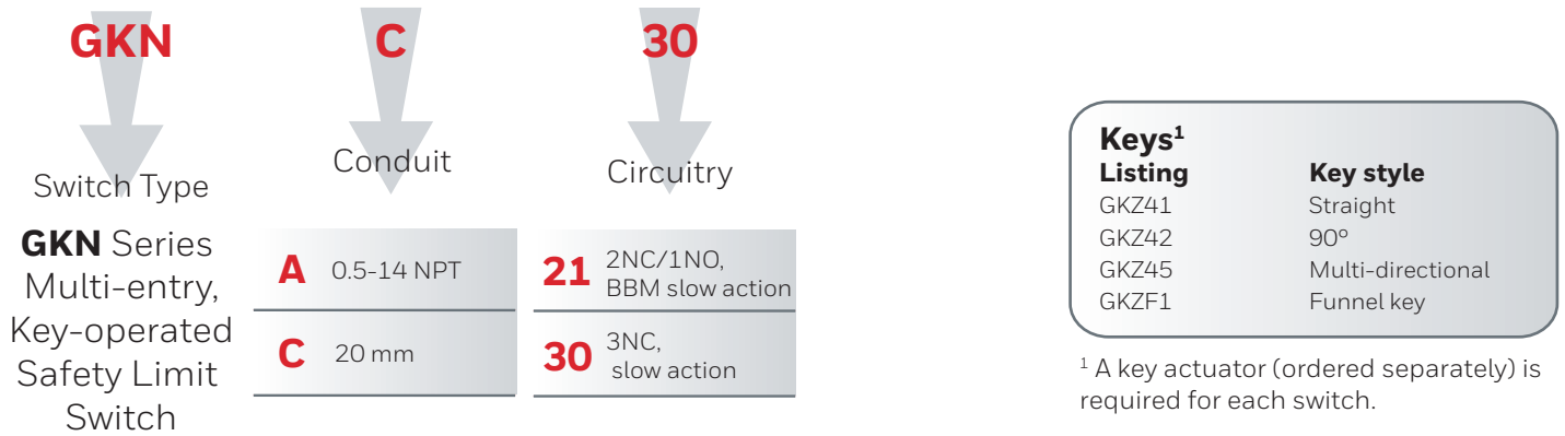
Figure 1. Product Nomenclature
