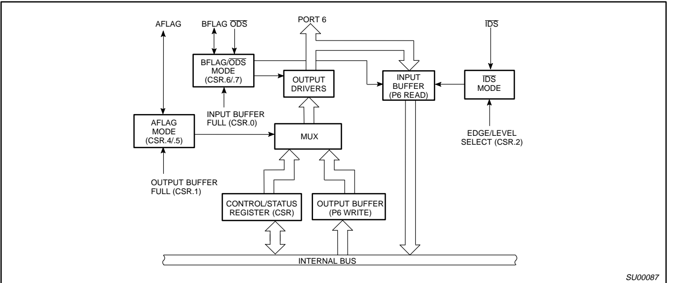
Figure 8. Port 6 Block Diagram
