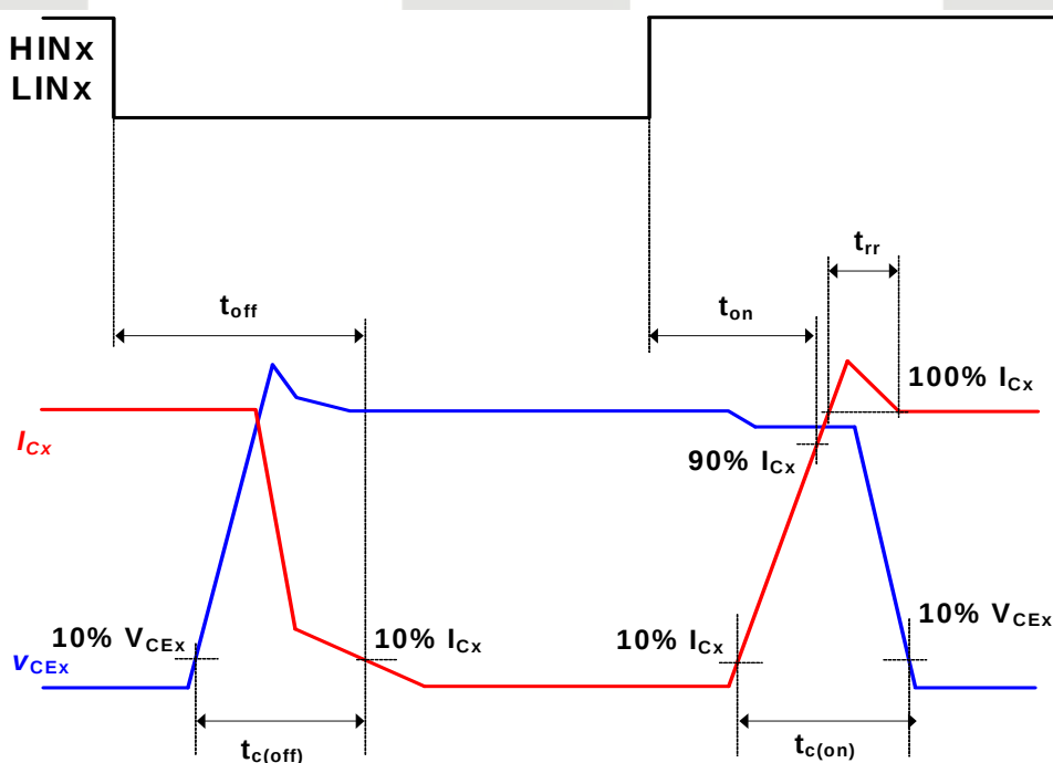
Figure 4. Switching Time
