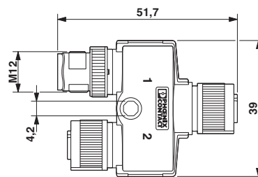
Dimensioned drawing
