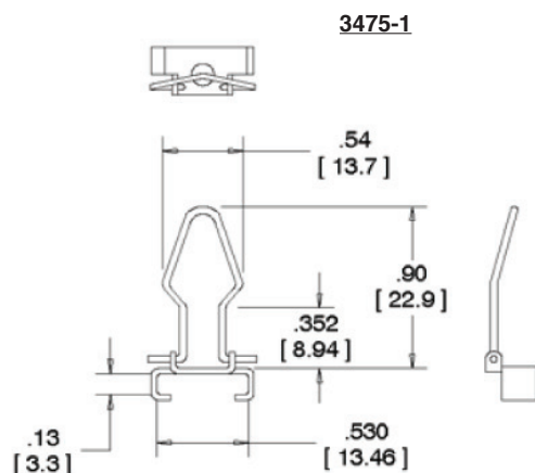
Plastic Connectors Mounted to Front of Panel
