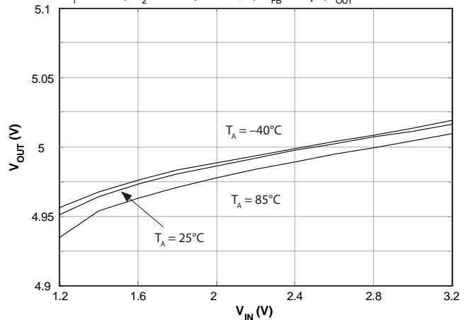
Line Regulation — PWM Mode ( V_{OUT} = 5.0V )
