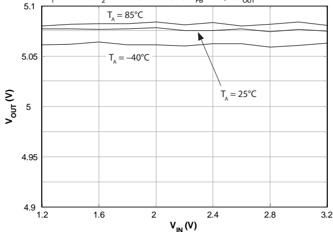
Line Regulation — PSAVE Mode ( V_{OUT} = 5.0V )
