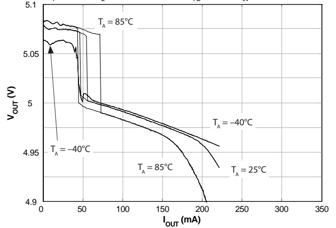
Load Regulation ( V_{OUT} = 5.0V )
