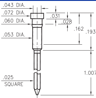
1302-0-05-XX-00-00-01-0 Press-fit in .057 mounting hole
