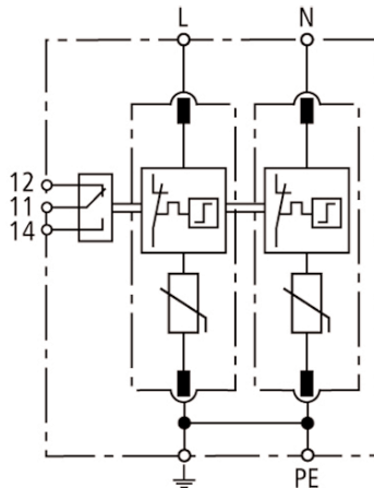
BSPM2275TN(R)
