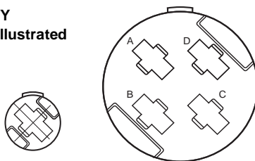
Tri-Start (MIL-DTL-38999, Series III) Connectors with MT Ferrule Inserts
