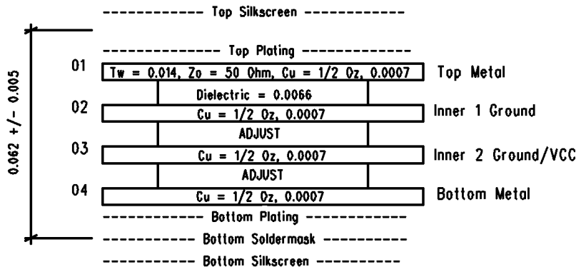
Figure 10. QFN-48 Evaluation Board Layout, 4-Layer Stack
