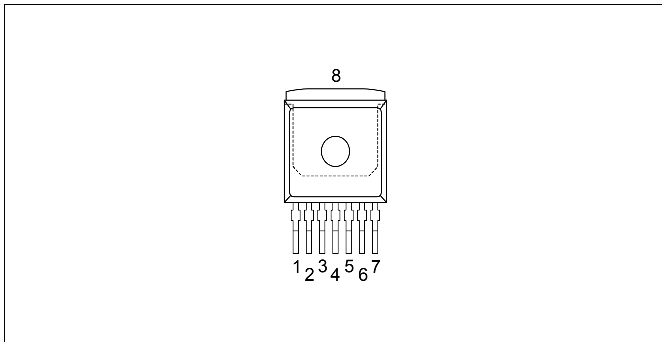
Figure 3 Pin Assignment BTN8962TA (top view)
