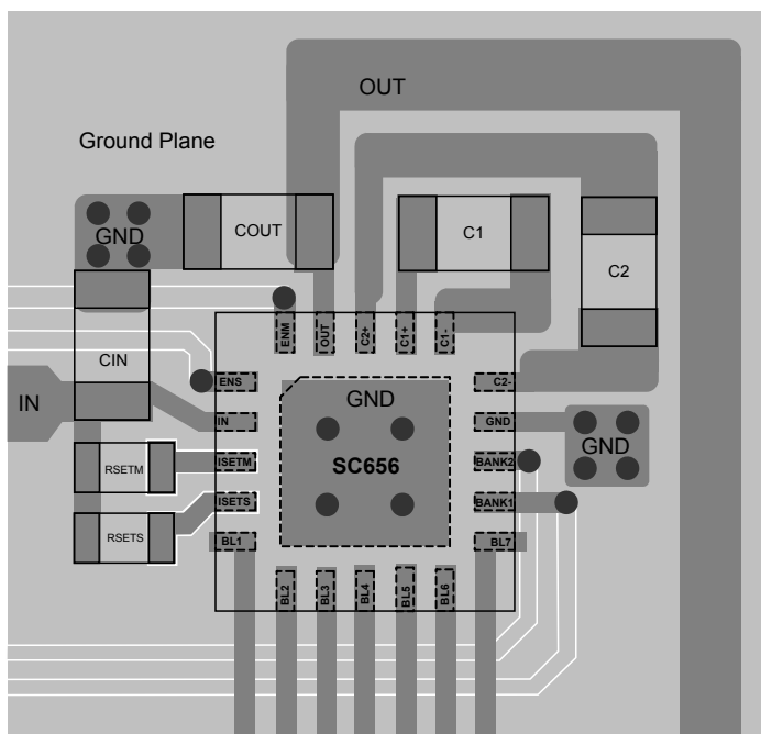
Figure 2 — Recommended Layout
