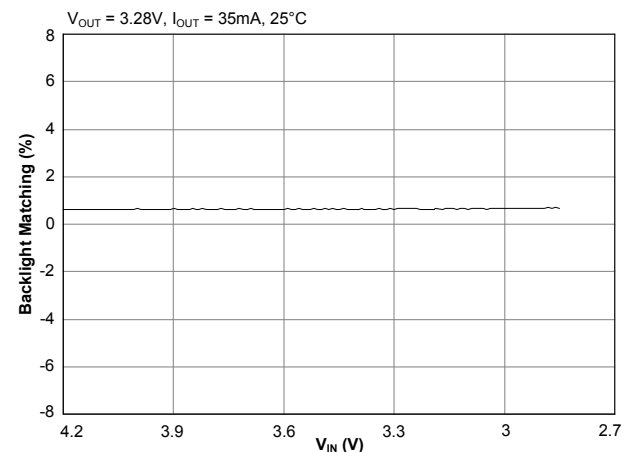
Backlight Matching (7 LEDs) — 5mA Each
