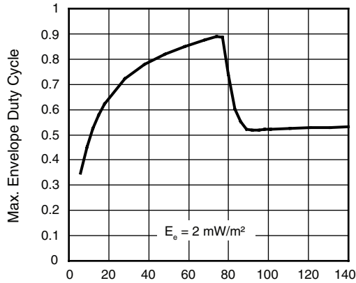
21396_1 Burst Length (number of cycles/burst) Fig. 9 - Max. Envelope Duty Cycle vs. Burst Length
