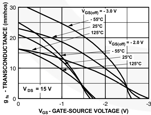
Figure 7. Transfer Characteristics
