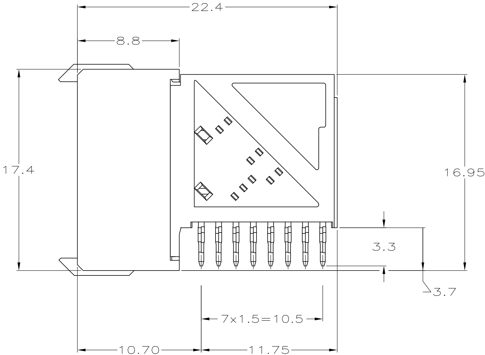
SECTION W-W
