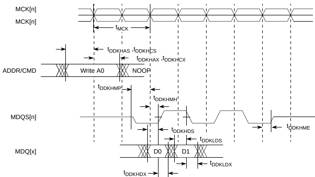
Figure 5. DDR2 and DDR3 SDRAM Interface Output Timing Diagram
