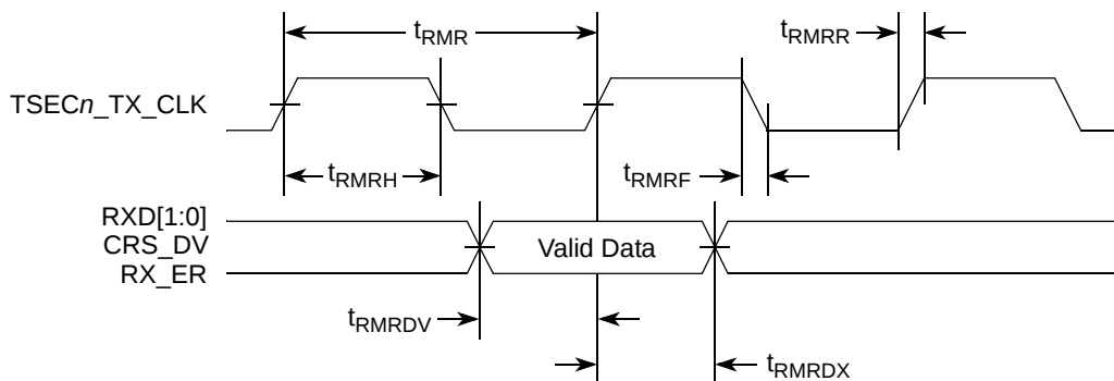
Figure 21. RMI Receive AC Timing Diagram
