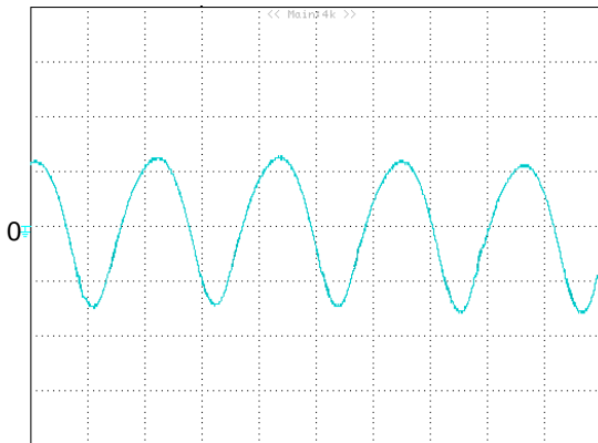
Figure 12: Output voltage ripple at nominal input voltage ( V_{in}=48\text{V} ) and rated load current ( 50\ \text{mV}/\text{div} , 2\ \mu\text{s}/\text{div} ). Load capacitance: 1\ \mu\text{F} ceramic capacitor and 10\ \mu\text{F} tantalum capacitor. Bandwidth: 20\ \text{MHz} . Scope measurements should be made using a BNC cable (length shorter than 20 inches). Position the load between 51 mm to 76 mm (2 inches to 3 inches) from the module
