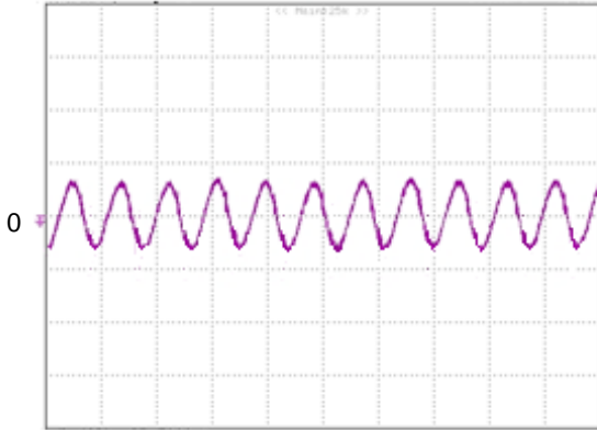
Figure 10: Input reflected ripple current, i_s , through a 12\ \mu\text{H} source inductor at nominal input voltage ( V_{in}=48\text{V} ) and rated load current ( 20\ \text{mA}/\text{div} , 5\ \mu\text{s}/\text{div} )
