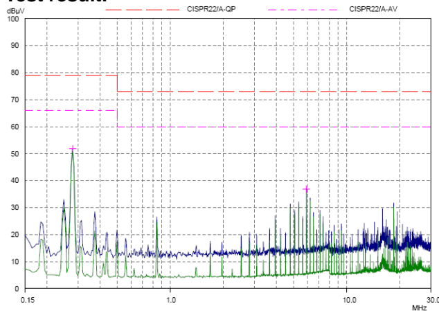
25C, 48Vin, full load, Green line is quasi peak mode and blue line is average mode.
