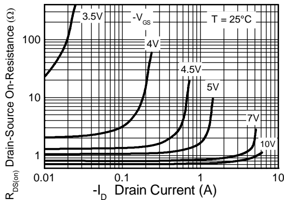
On-Resistance v Drain Current
