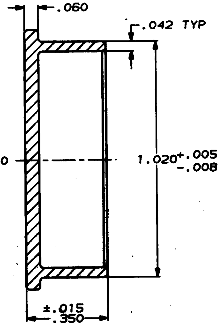
SECTION T-T
