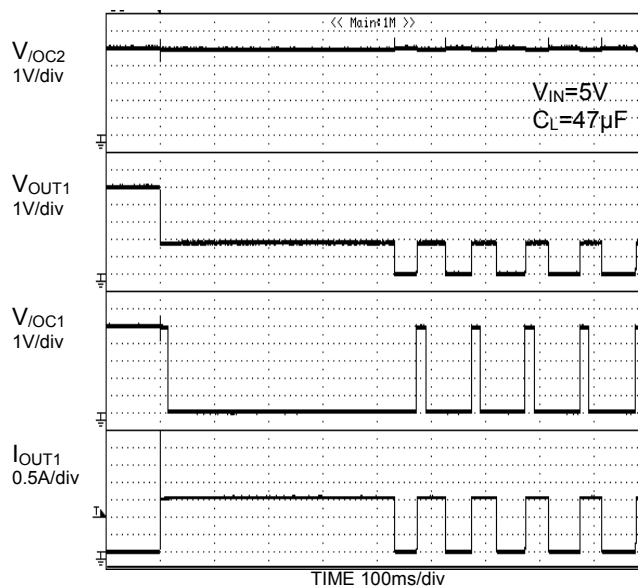
Figure 37. Thermal Shutdown Response (BD2062FJ)
