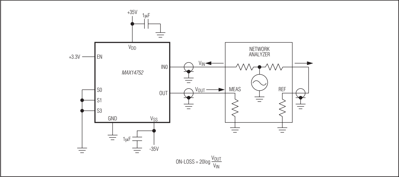
Figure 7. Frequency Response
