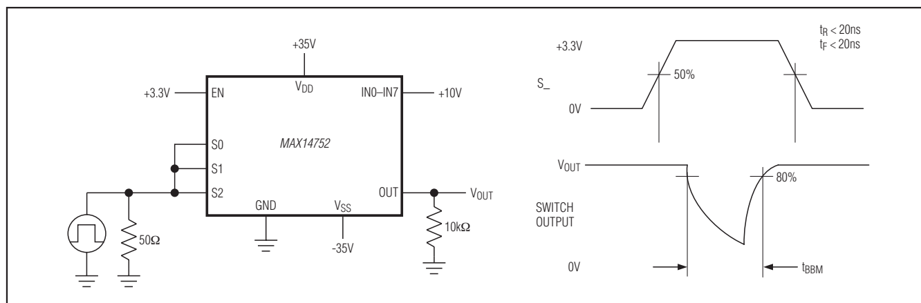
Figure 6. Break-Before-Make Interval
