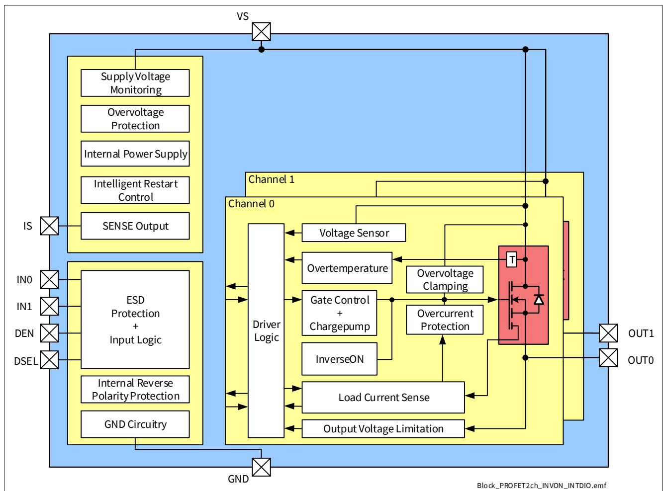
Figure 2 Block Diagram of BTS7120-2EPA
