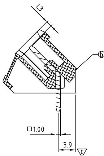
SECTION P-Q
