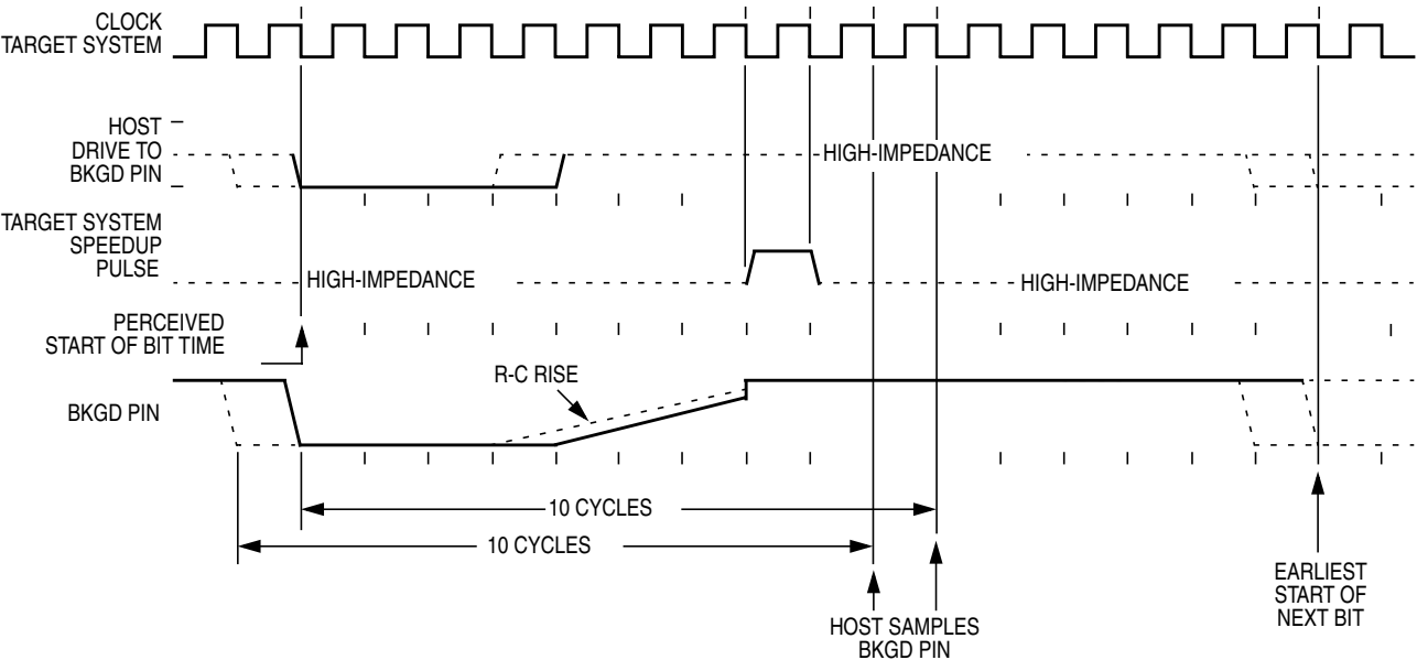
Figure 6-8. BDM Target-to-Host Serial Bit Timing (Logic 1)
