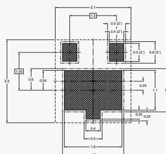
DFN2020-3 (SOT1061)
