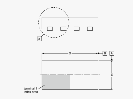
DFN2111-7 (SOT1358)
