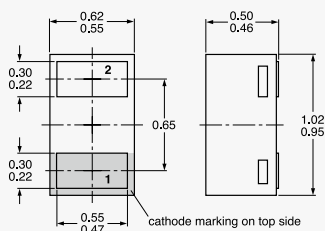
DFN1006-2 (SOD882)
