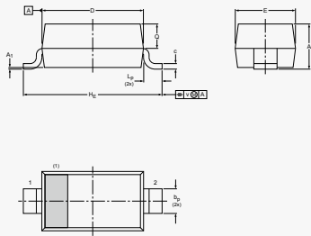
SOD123
