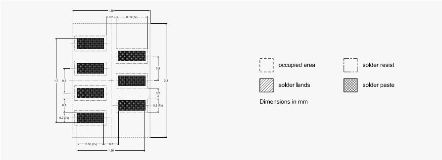
DFN2111-7 (SOT1358)
