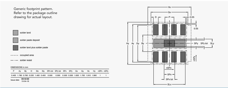
DFN1714U-8 (SOT983)
