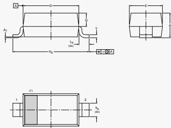
SOD123
