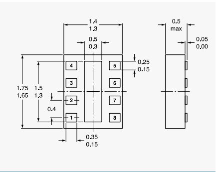
DFN1714U-8 (SOT983)
