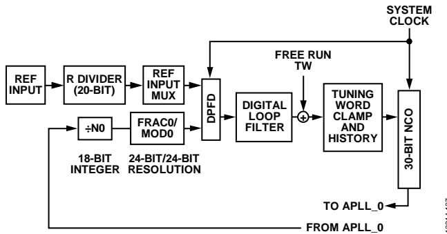
Figure 27. DPLL_0 Core
