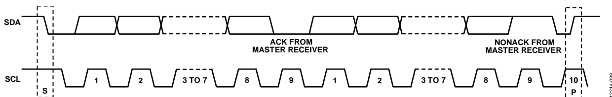
Figure 42. Data Transfer Process (Master Read Mode, 2-Byte Transfer), First Acknowledge From Slave
