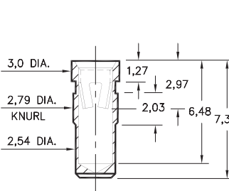
5834-0-15-XX-23-XX-10-0 Press-fit in 2,72 mounting hole
