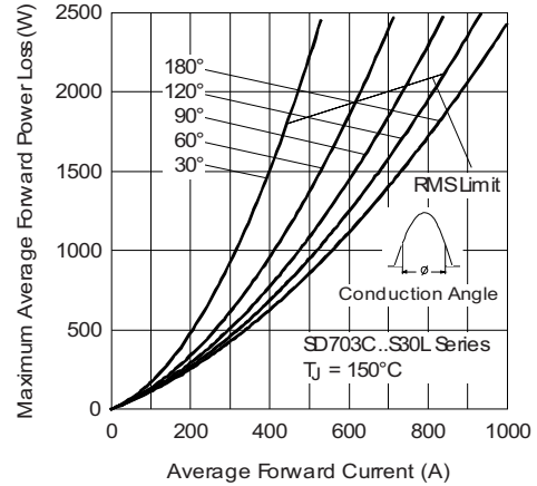
Fig. 11 - Forward Power Loss Characteristics
