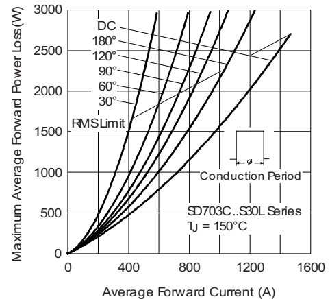
Fig. 12 - Forward Power Loss Characteristics
