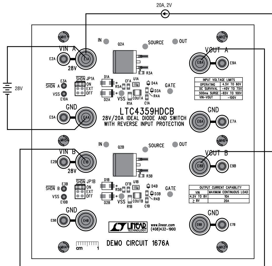
Figure 6. Testing Forward Drops without the Need for a High Power Supply or High Power Load.
