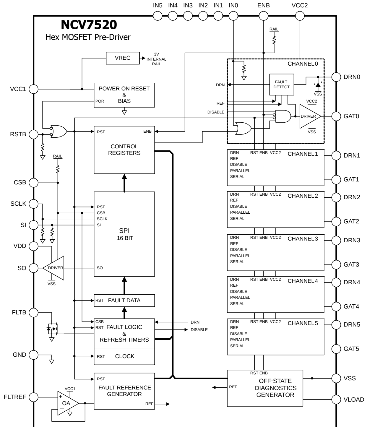
Figure 1. Block Diagram
