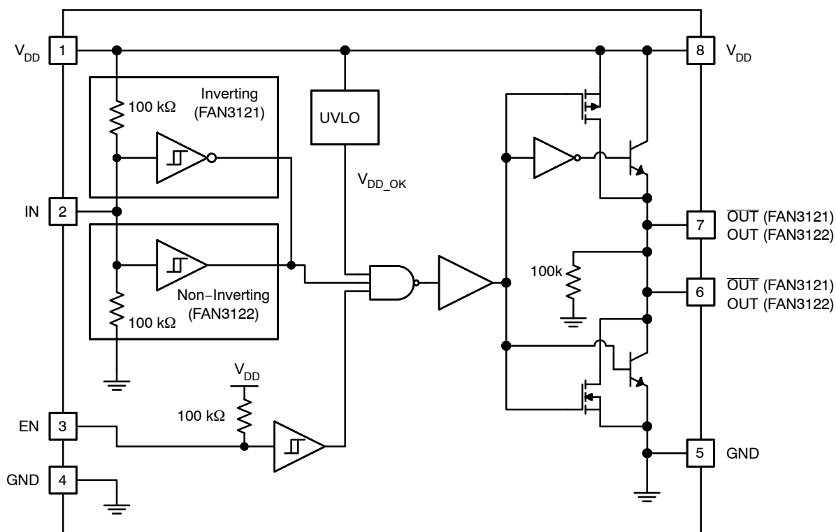
Figure 7. Block Diagram
