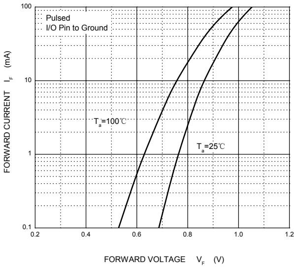
Forward Characteristics
