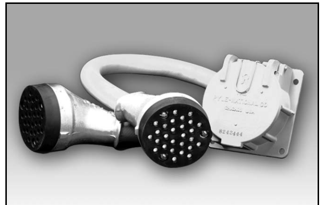
Amphenol® 27 Pole Train-line Receptacle and Jumpers for Rail Mass Transit
