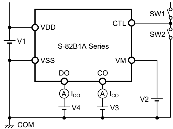
Figure 7 Test Circuit 4
