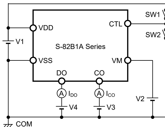
Figure 7 Test Circuit 4
