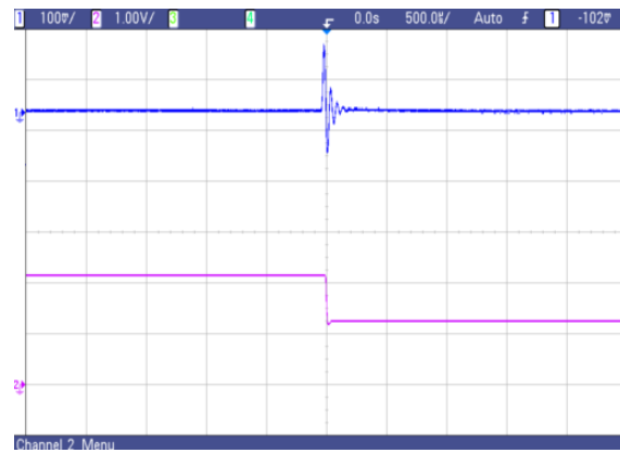
Fig. 24 AVO75-48S1V5 typical transient response to step decrease in load from 50% to 25% of full load, room temperature, 48Vdc input
