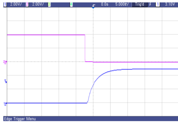
Fig. 68 AVO75-48S05 typical start-up from CNT on
