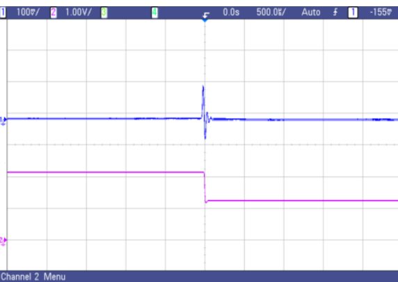
Fig. 32 AVO75-48S1V8 typical transient response to step decrease in load from 50% to 25% of full load, room temperature, 48Vdc input ( \Delta I_o/\Delta t=1A/1\mu s )
