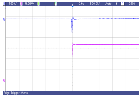
Fig. 45 AVO75-48S05 typical transient response to step increase in load from 50% to 75% of full load, room temperature, 48Vdc input ( \Delta I_o/\Delta t=1A/1\mu s )
